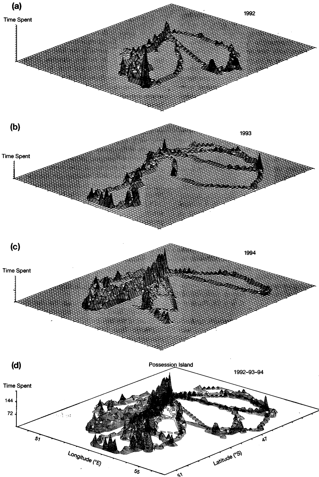
Fig. 1. Amount of time spent by king penguins in a 0.1^\circ \times 0.1^\circ grid around Possession Island (Crozet Archipelago) in the summers of (a) 1992, (b) 1993, (c) 1994 and (d) the 3 years pooled. Each unit of the vertical contours corresponds to 30 min
