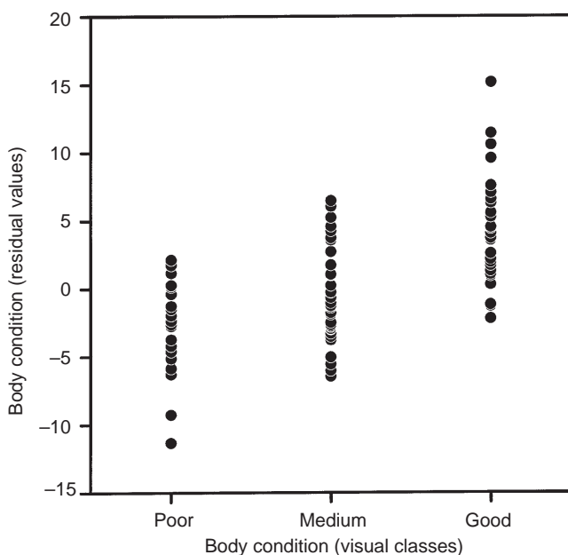
Fig. 2. Validation of the visually evaluated maternal body condition indices using residual values of the linear regression between maternal body mass and body length (see Methods).
