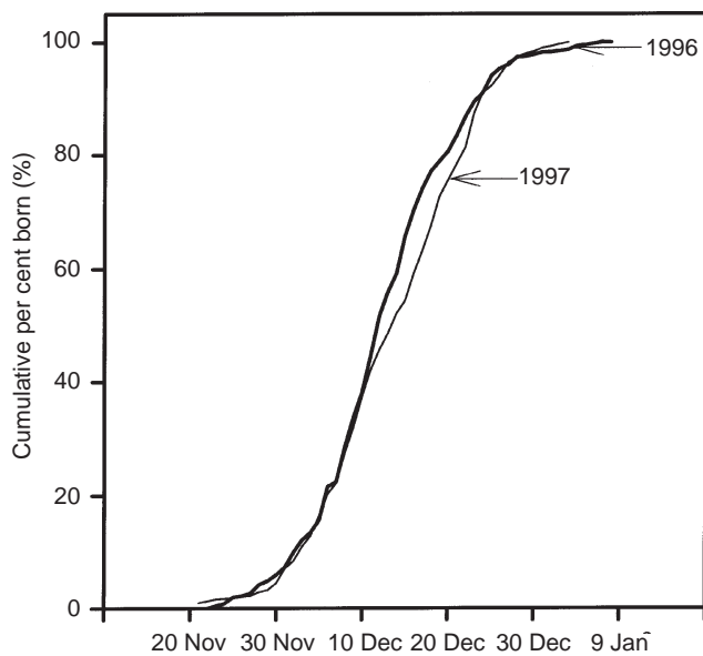
Fig. 4. Cumulative percentage of pups born in relation to date for the 1996 (heavy line) and 1997 (light line) reproductive seasons.
