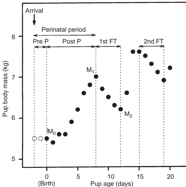
Fig. 3. Schematic representation of the perinatal period with a typical example of records of pup mass changes from birth until a few days after the first foraging trip in a subantarctic fur seal pup (female pup J165 born on 3 December 1997). Mother arrived 2 days before giving birth (pre P: prenatal period). During the postnatal period (Post P), pup body mass was M_0 at birth, decreased typically during the first day of life and then increased to pup body mass after the postnatal period ( M_1 ), corresponding to an absolute pup mass gain M_1 - M_0 . Pup growth rate during the postnatal period was defined by [M_1 - M_0] / \text{Post P} . During the first foraging trip (1st FT), the pup fasted and lost mass until M_2 , when mother came back ashore.
