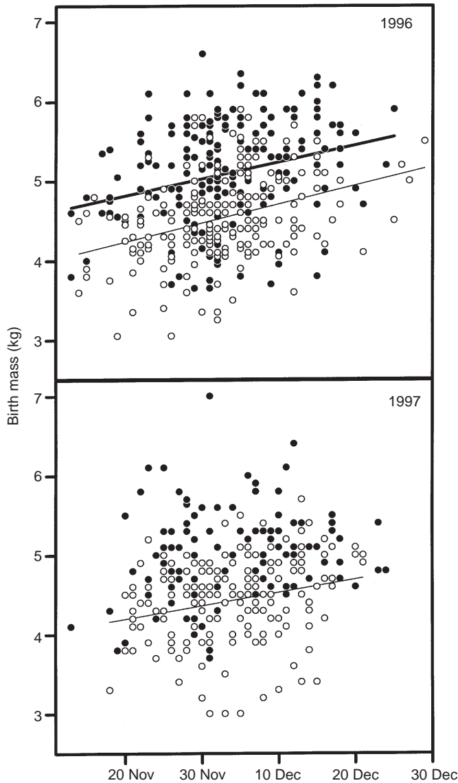
Fig. 5. The relationship between birth date and birth mass in male (closed circles) and female (open circles) pups for the 1996 and 1997 reproductive seasons.
