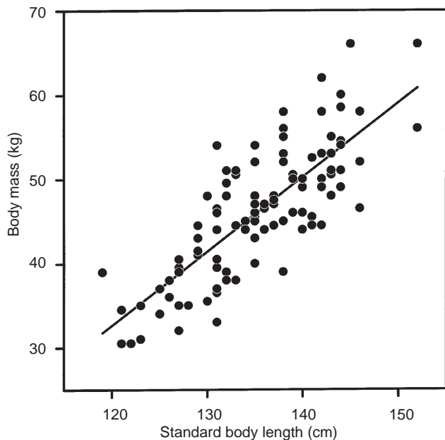
Fig. 1. Linear relationship between body mass and standard body length in lactating subantarctic fur seals breeding on Amsterdam Island during the 1996 reproductive season. Maternal body condition was determined using residual values of this regression.
